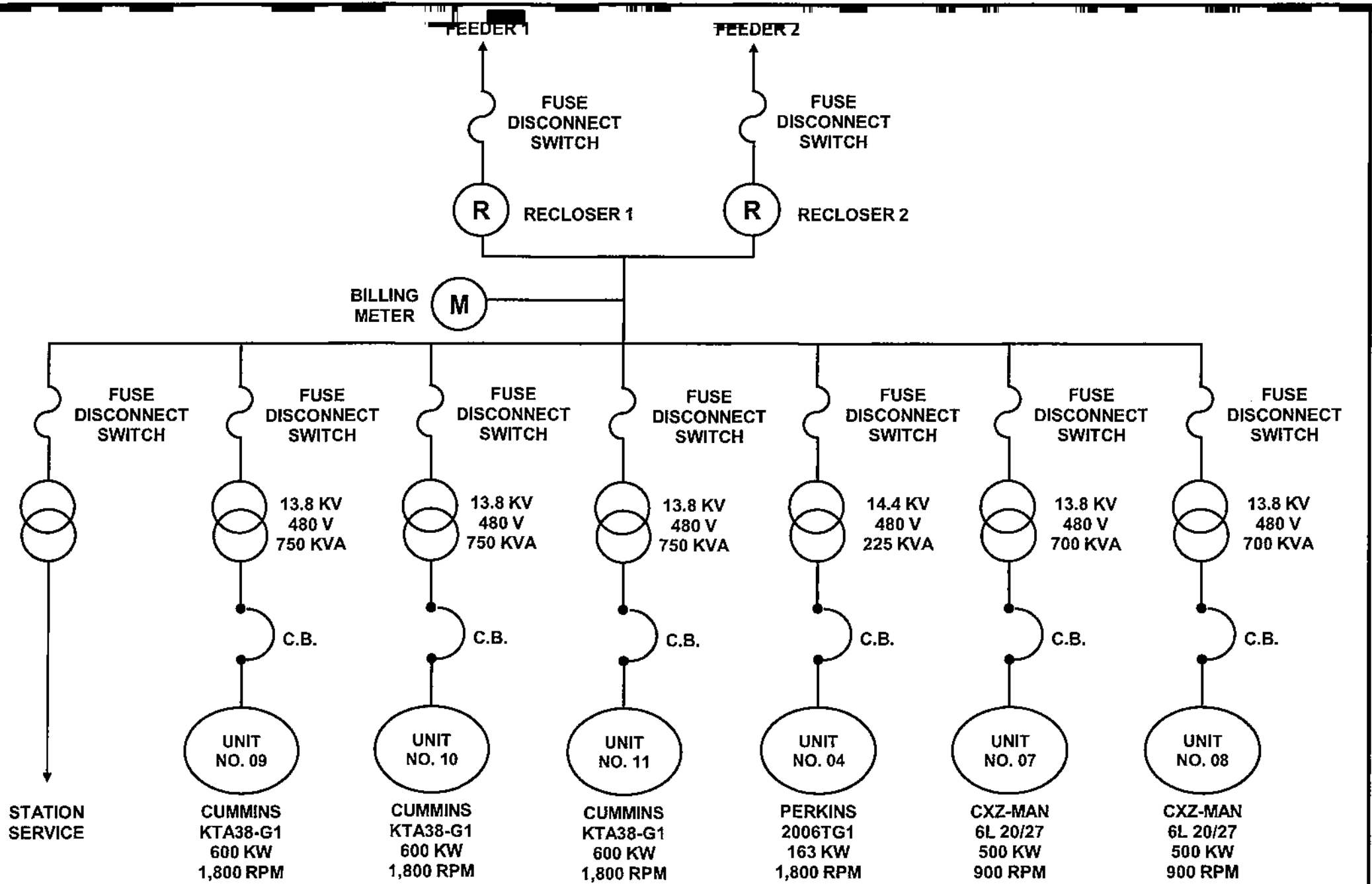
SIBUYAN DIESEL POWER PLANT SINGLE LINE DIAGRAM
